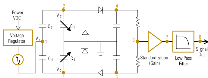
Figure 3: Circuit Schematic
