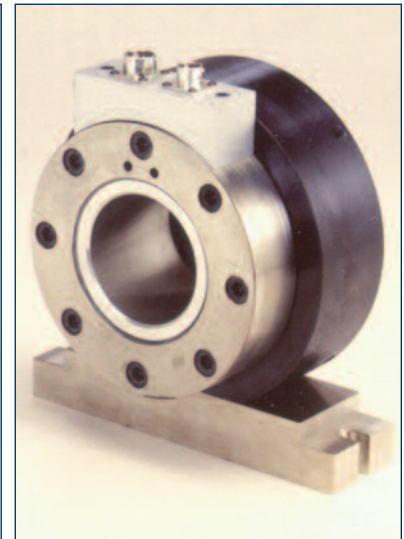
Series FTA9000 Torque-Tension Load Cell
