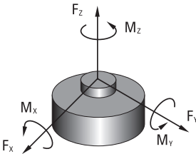
Figure 3a: Right-handed Orthogonal Coordinate System
