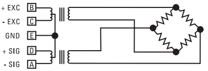
Figure 2b: Wiring Code
