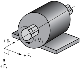
Figure 4: Axis and Sense Nomenclature for Torque Sensors
