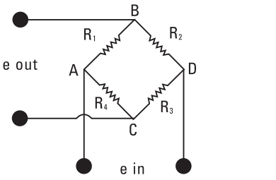
Figure 1: Wheatstone Bridge
