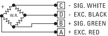
Figure 2a: Wiring Code
