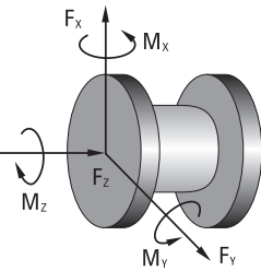
Figure 3b: Right-handed Orthogonal Coordinate System
