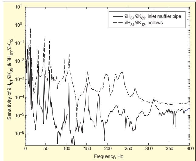
Figure 9. Comparison of stiffness sensitivity functions of the exhaust system to changes near the bellows and the inlet muffler pipe.
