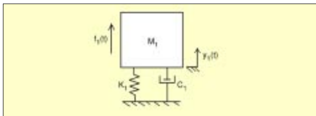
Figure 1. Schematic of a single degree-of-freedom linear system model.
