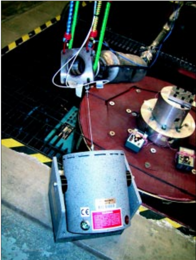
Figure 6. Electrodynamic shaker attached with stinger to front bracket of exhaust system in front of the bellows to simulate input from powertrain.
