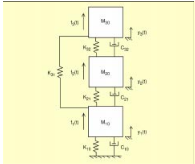
Figure 3. Schematic of a three degree-of-freedom linear system model with an alternative parameter labeling format used to emphasize coupling.
