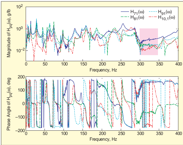
Figure 11. Magnitude (upper) and phase (lower) of y-direction FRFs of the modified exhaust with Metex joint.
