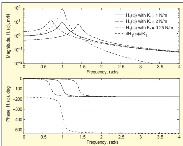
Figure 2. Magnitude (upper) and phase (lower) plots of single degree-of-freedom frequency response function for three values of K_1 with the corresponding embedded sensitivity function \partial H_1 / \partial K_1 for the system stiffness parameter.
