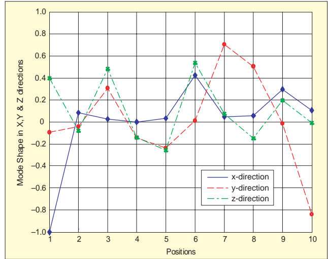
Figure 8. Relative deflection mode shapes in x-, y- and z-directions estimated using the imaginary parts (peak-pick method) of the associated FRFs (normalized).
