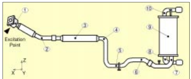
Figure 5. Illustration of measurement degrees-of-freedom used in tests on exhaust subsystem; triaxial acceleration measurements were made at each point.
