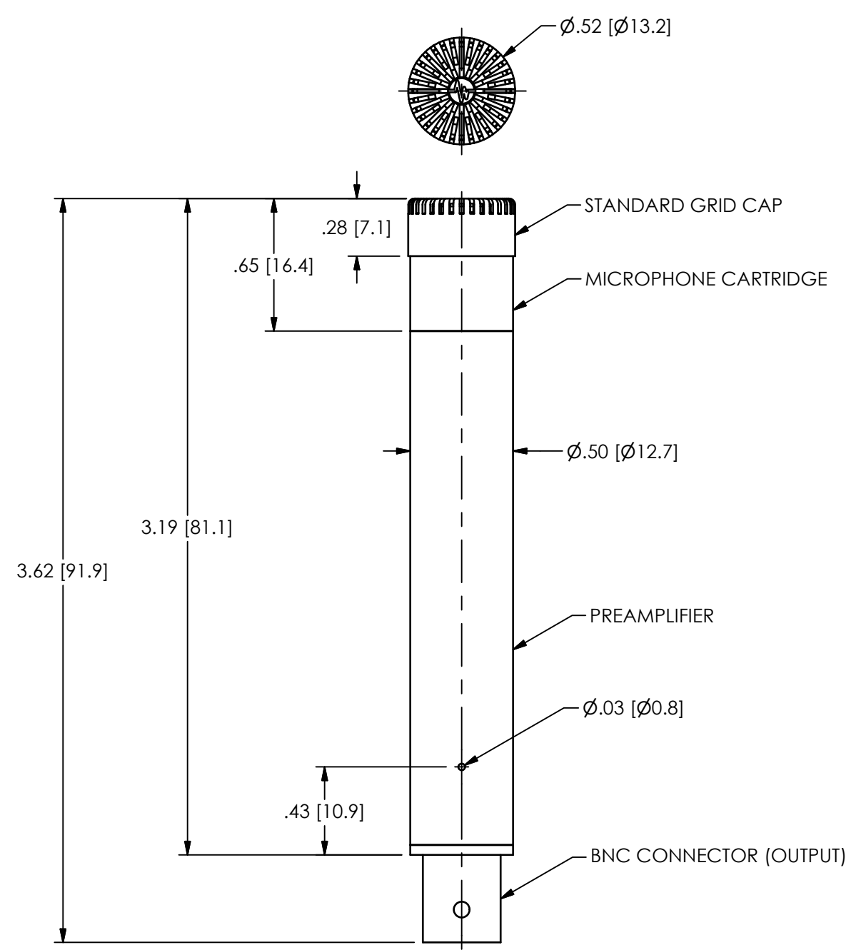
STANDARD GRID CAP INSTALLED
