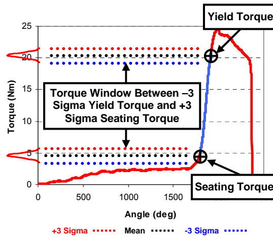
Figure 23: Torque Window Using Seating Torque
