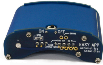
AT-5000 End View (showing gain resistor, shunt cal connector, and gage connections)
