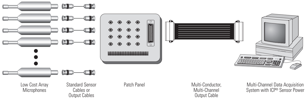
Figure 31. Array Microphone System
