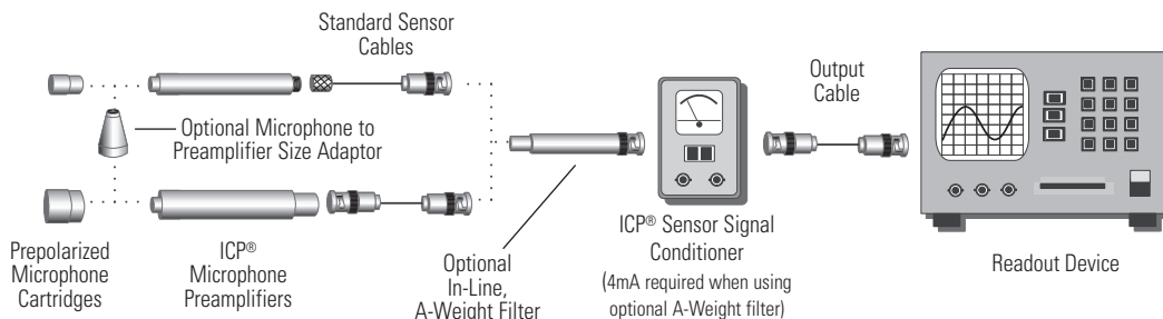
Figure 30. Prepolarized Microphone System
