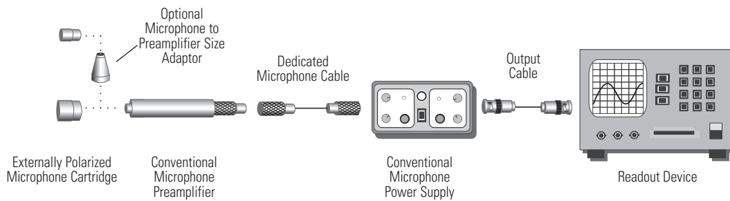
Figure 29. Externally Polarized Microphone System
