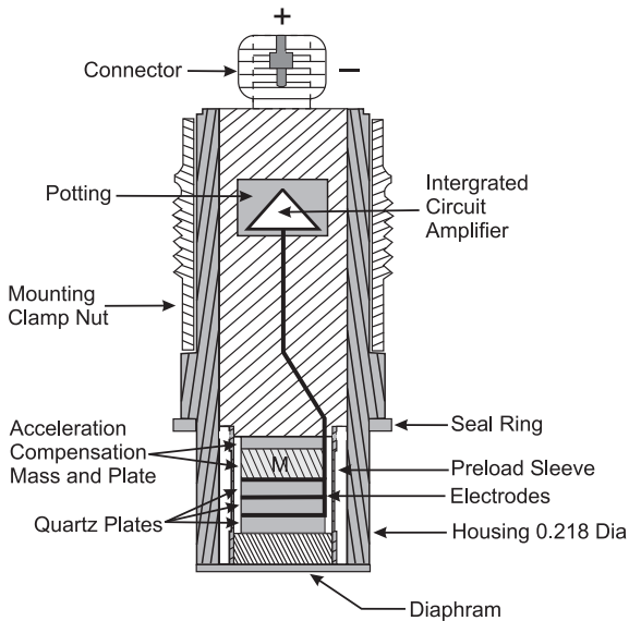
Figure 32. Typical ICP Quartz Pressure Sensor
