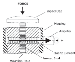
Figure 36. Compression-Tension-Impact Series 208
