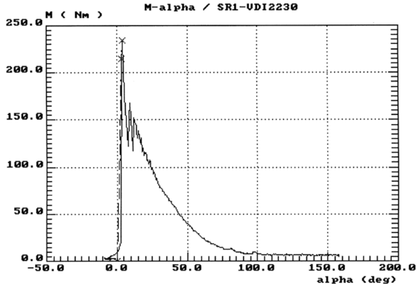
Figure 16. Wheel nut Loosening Signature
