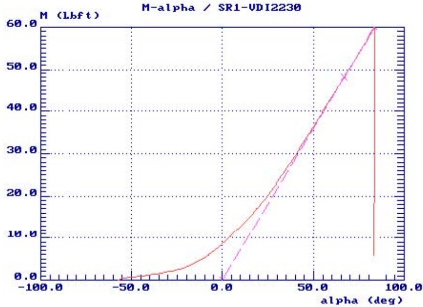
Figure 20. M-Alpha Diagram
