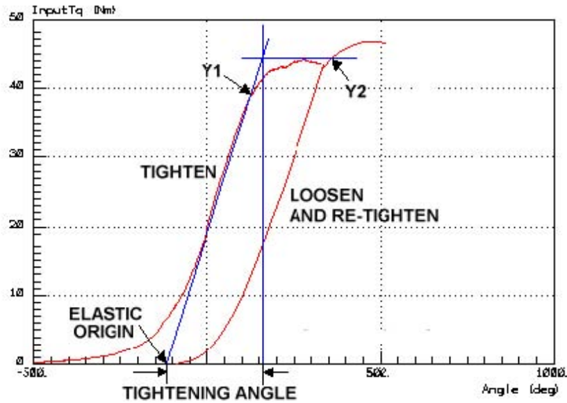
Figure 8. Bolt Yield
