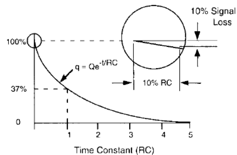
Figure 6b Linear Portion of a DC Coupled Discharge Time Constant
