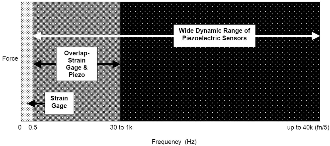
Figure 6 Technology Overlap – Quartz Piezoelectric versus Strain Gage
